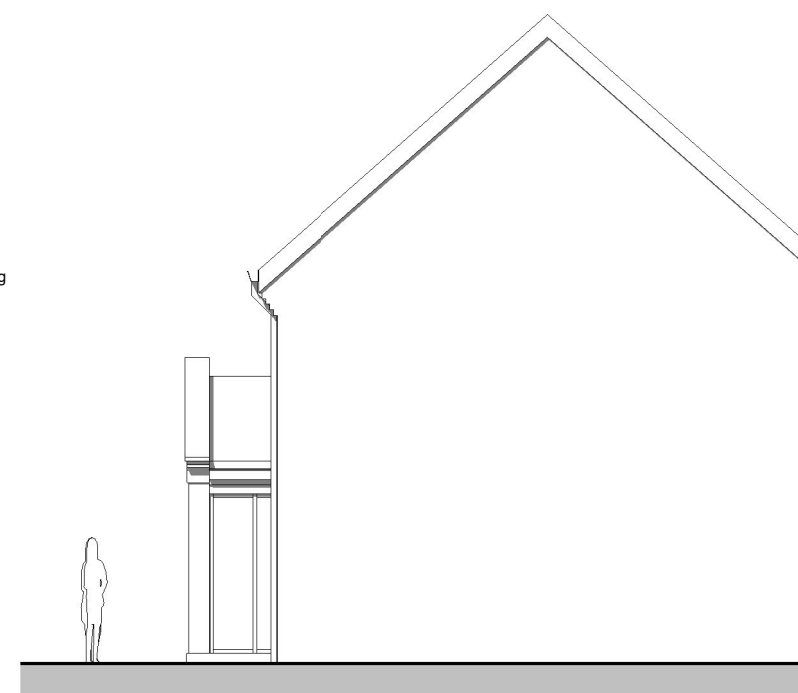
West Elevation 1 : 100
